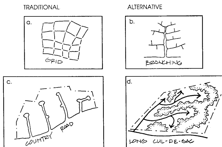
FIGURE 22. STREET LAYOUT EXAMPLES
