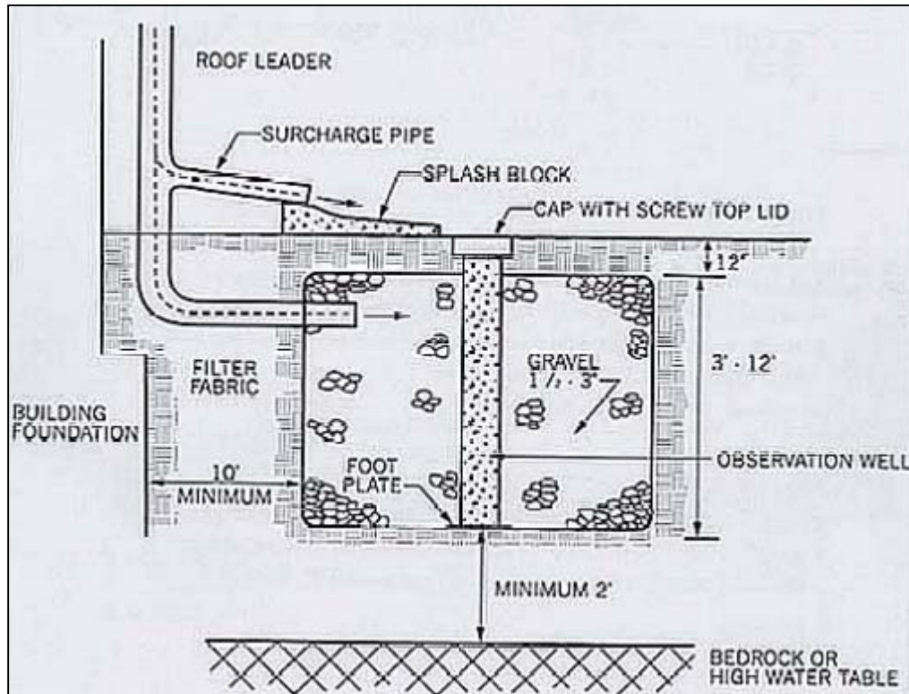
FIGURE 3. DRY WELL
